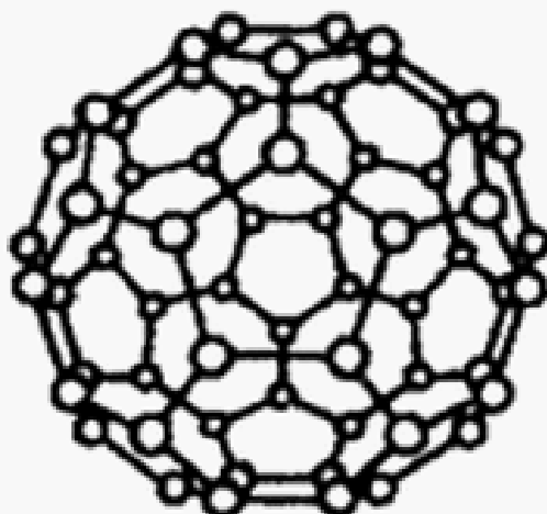
C_{60}
