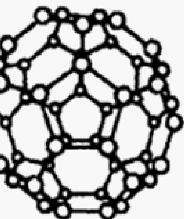
C_{50}
