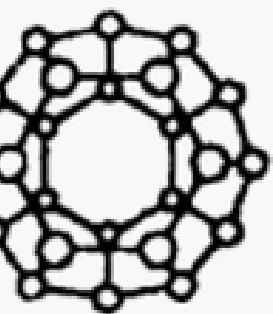
C_{24}
